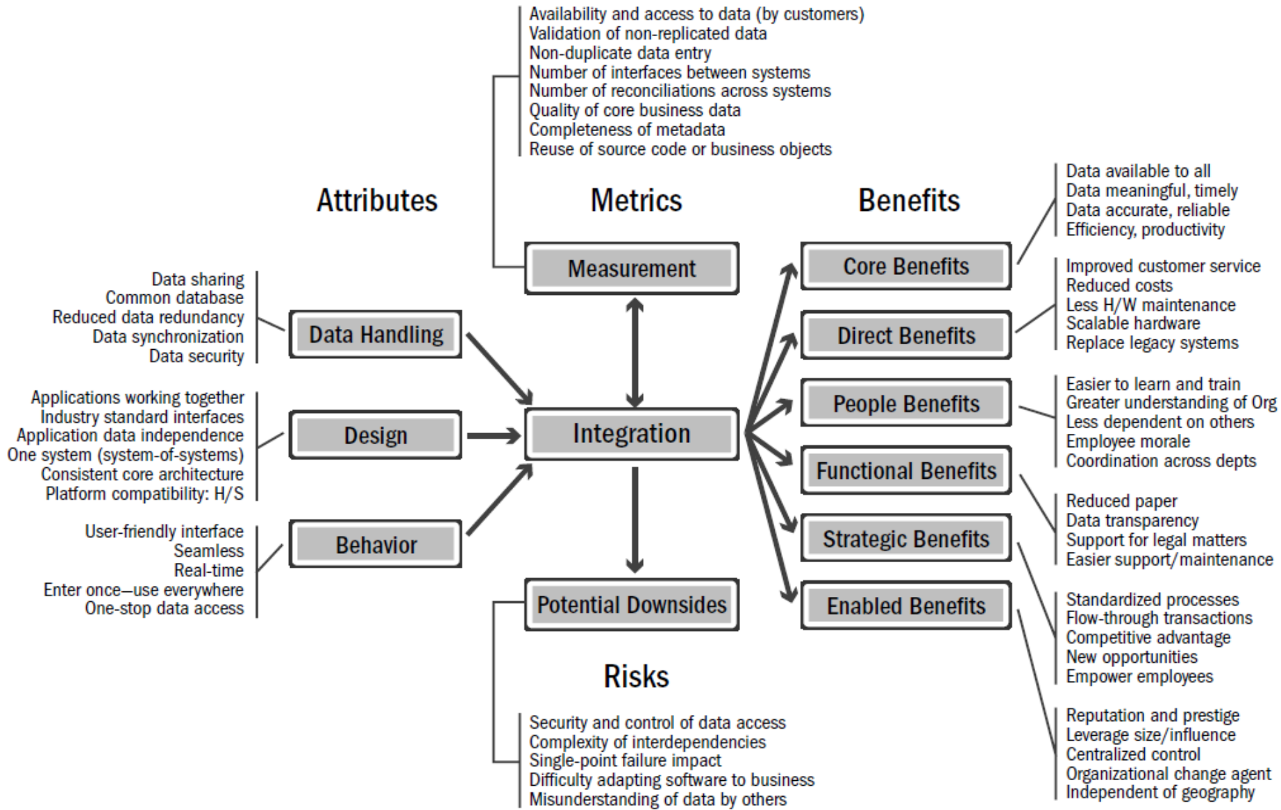
Figure 1.1 Definition of integration
